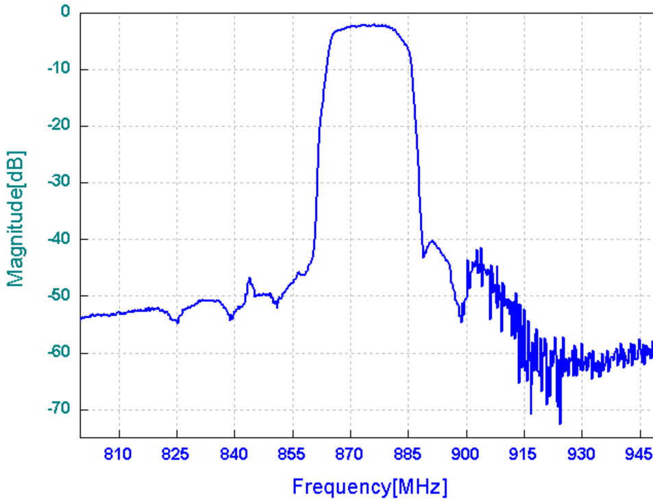
Frequency Response
